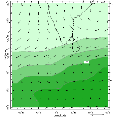
Time Mar Pressure 925.0 mb
