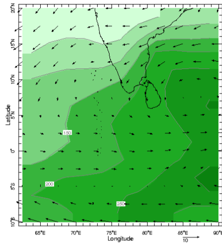
Time Nov Pressure 925.0 mb
