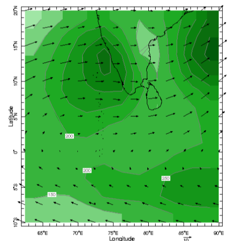
Time Jun Pressure 925.0 mb
