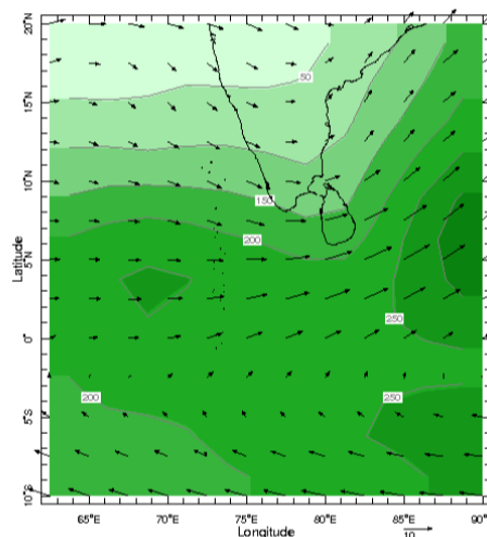
Time May Pressure 925.0 mb
