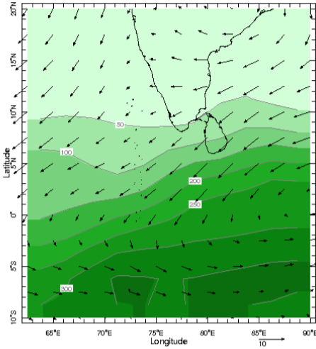
Time Jan Pressure 925.0 mb
