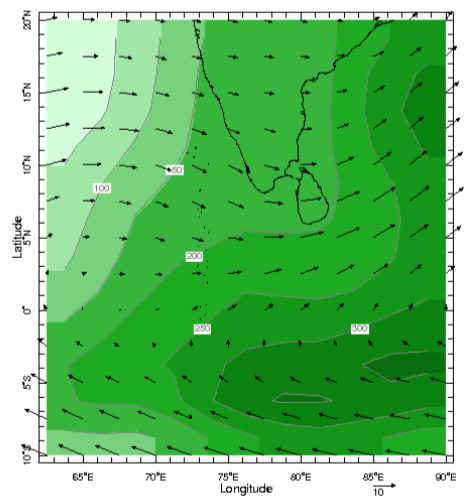
Time Sep Pressure 925.0 mb
