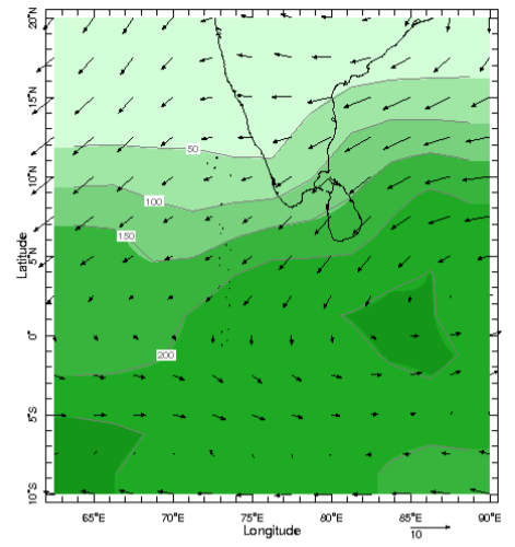
Time Dec Pressure 925.0 mb
