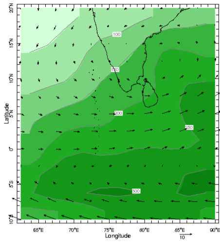
Time Oct Pressure 925.0 mb
