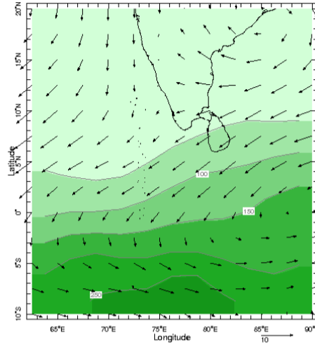
Time Feb Pressure 925.0 mb
