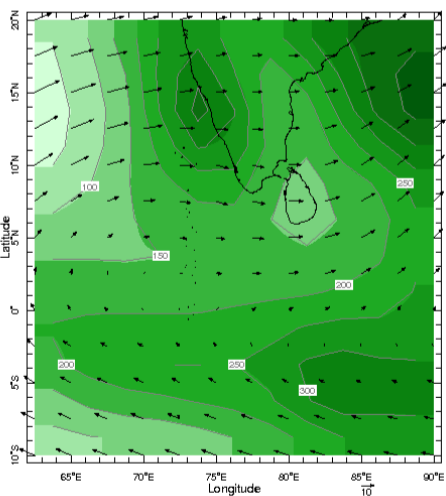
Time Jul Pressure 925.0 mb
