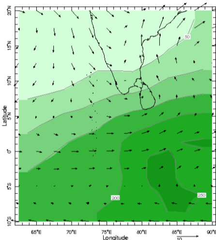
Time Apr Pressure 925.0 mb
