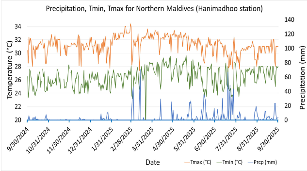
Daily Rainfall, Tmin & Tmax for the previous year in Hanimadhoo station (2024 September to 2025 September)
