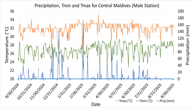
Daily Rainfall, Tmin & Tmax for the previous year in Male station (2024 September to 2025 September)
