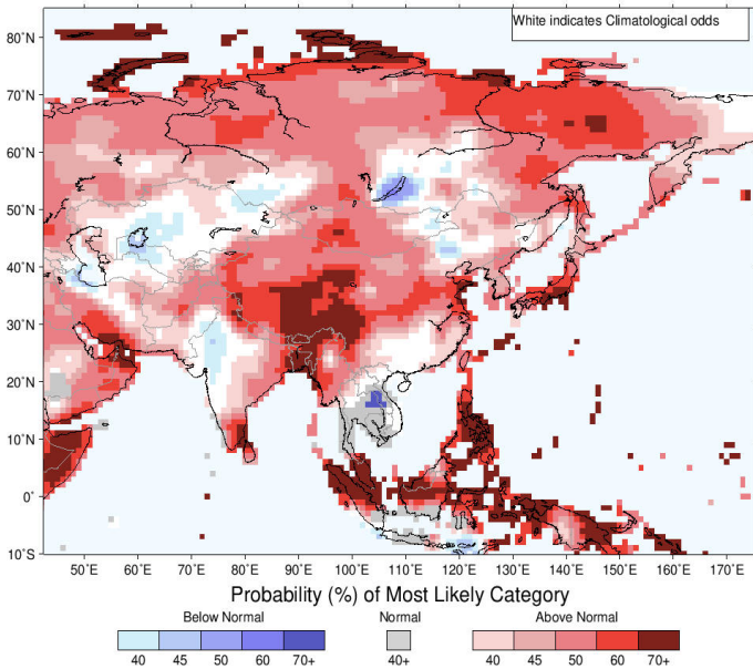
IRI Multi-Model Probability Forecast for Temperature for October–November–December 2025, Issued September 2025
