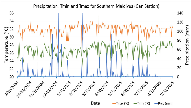
Daily Rainfall, Tmin & Tmax for the previous year in Gan station (2024 September to 2025 September)
